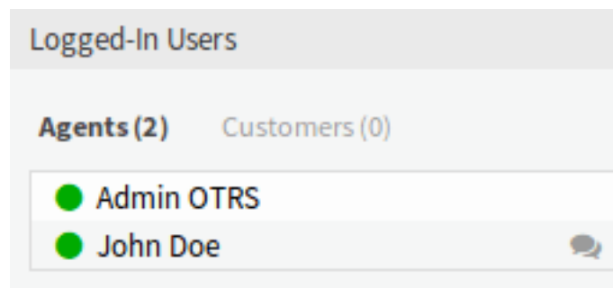
Fig. 8.2: Available Agents
