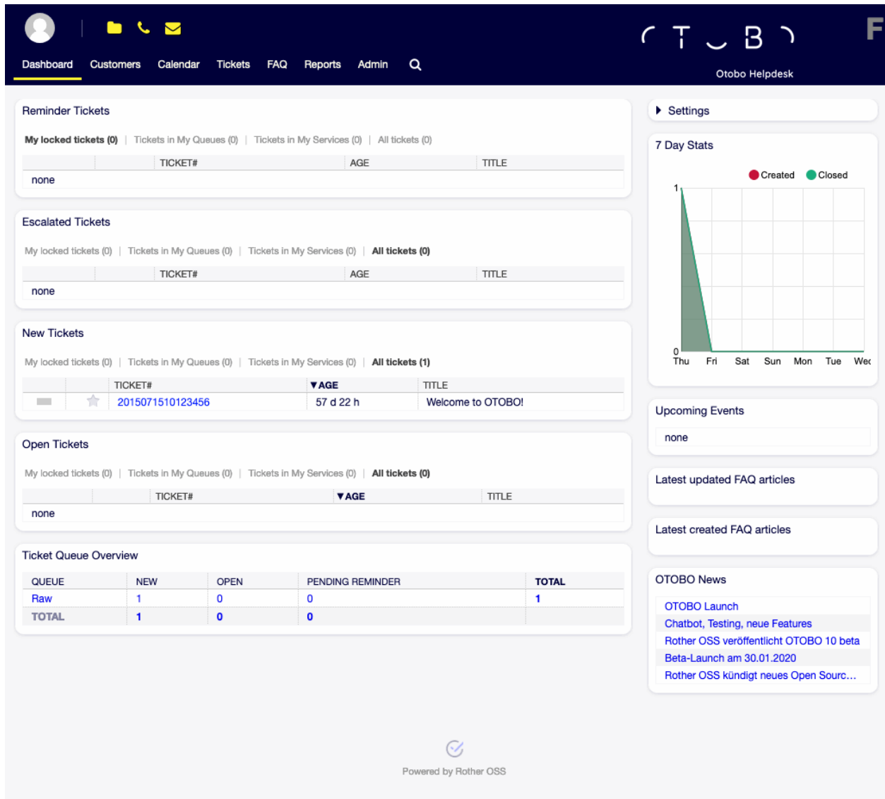
Fig. 2.1: Agent Dashboard
