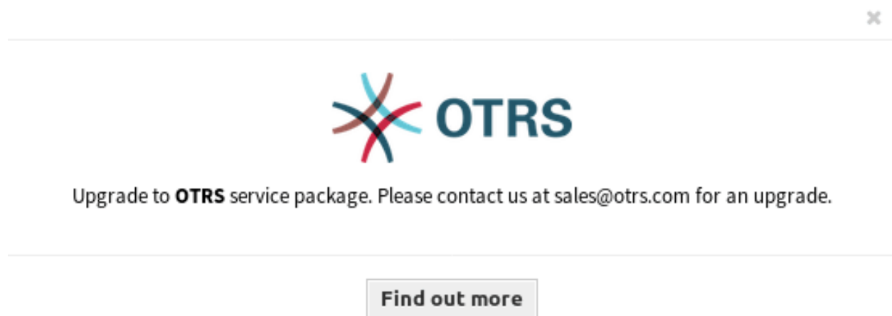
Fig. 5.8: Upgrade Dialog
