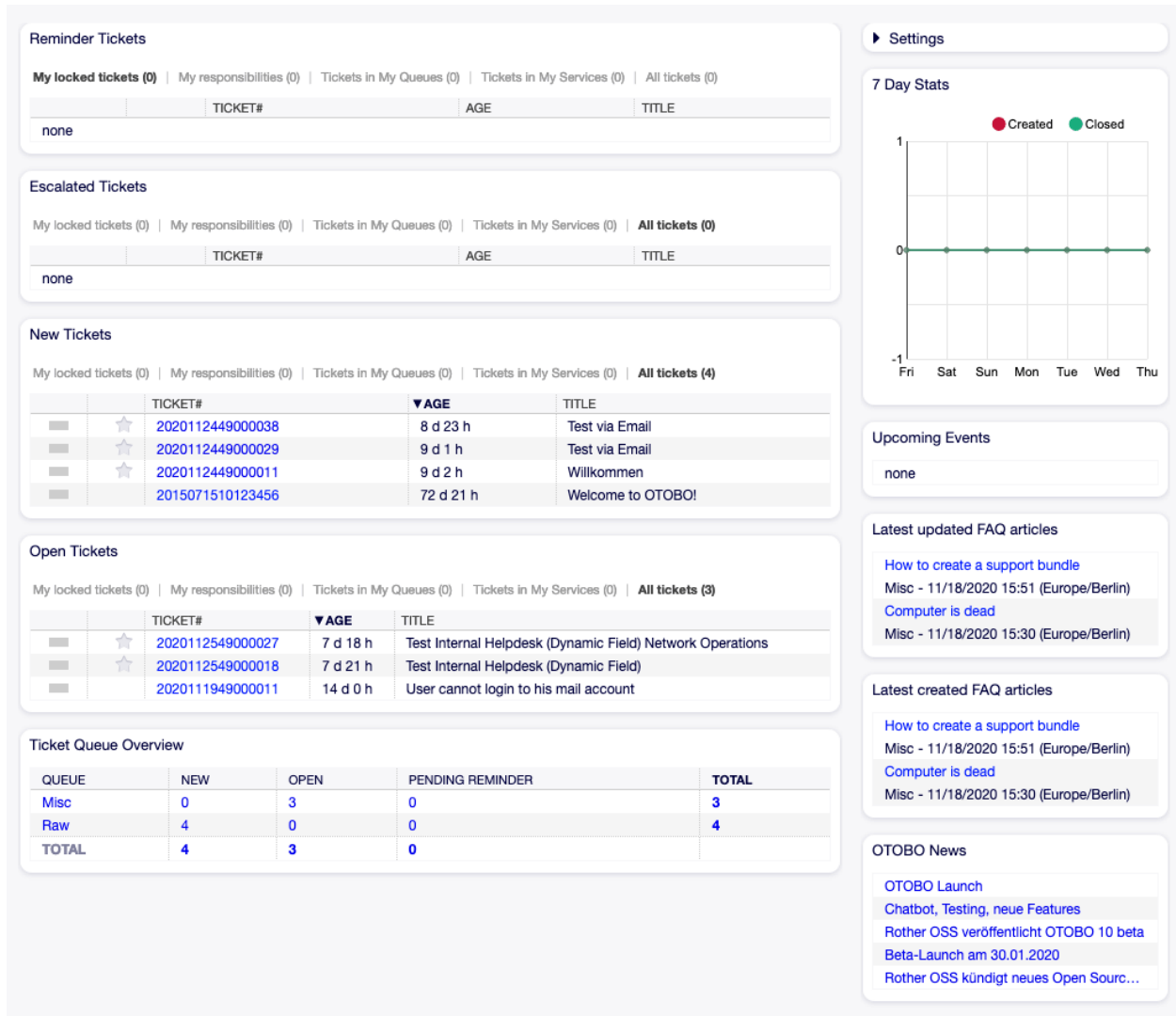
Fig. 2.3: Dashboard Widgets
