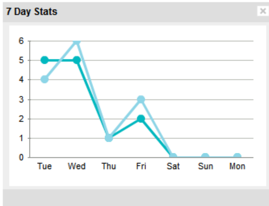
Figure 3.3: Dashboard Widget
