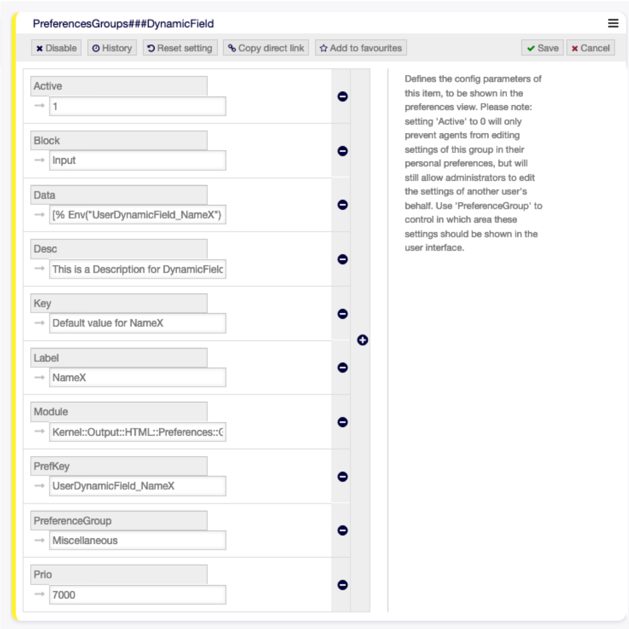
Fig. 5.32: Activate Dynamic Field in Personal Preferences
