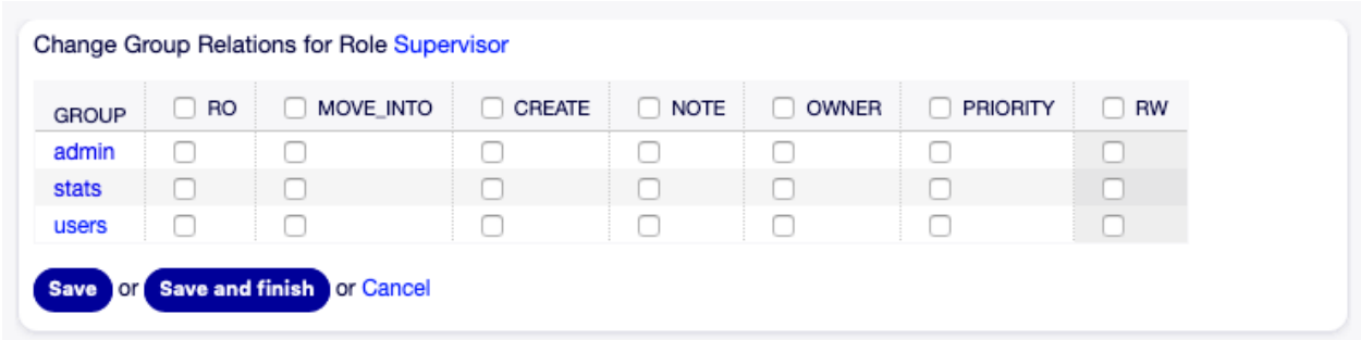
Fig. 4.43: Change Group Relations for Role
