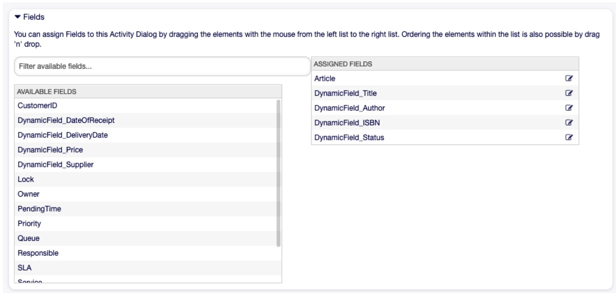
Fig. 5.50: Book Ordering - Add Activity Dialog Fields
